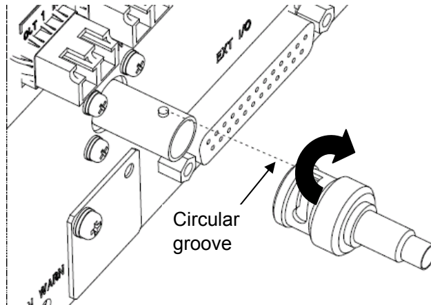
Figure 2-19 BNC Cable Connection
