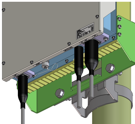
2.5GHz ODU
