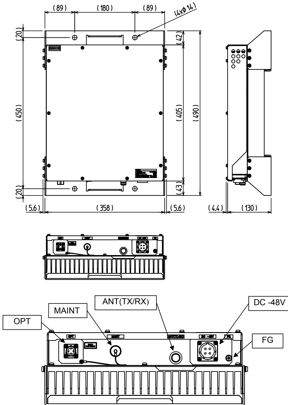
Figure 3-4 2.5GHz ODU Dimensions and Interface Part Details
