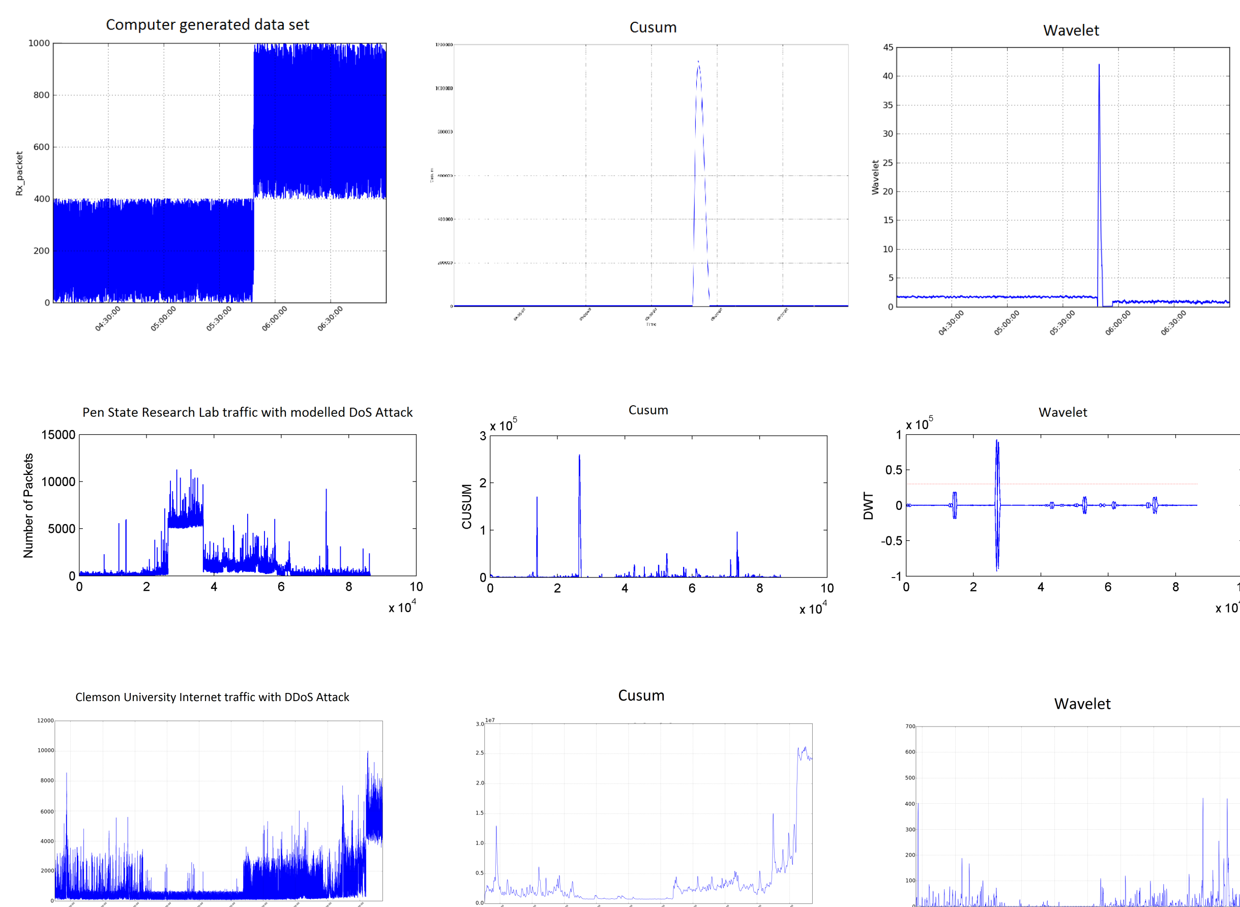
Fig 4. Detection results (Top) Computer generated data, its cusum and wavelet (Middle) Pen State firewall data with modelled attack, its cusum and wavelet (Bottom) Clemson Uni. Network traffic with DDoS attack, its cusum and wavelet
