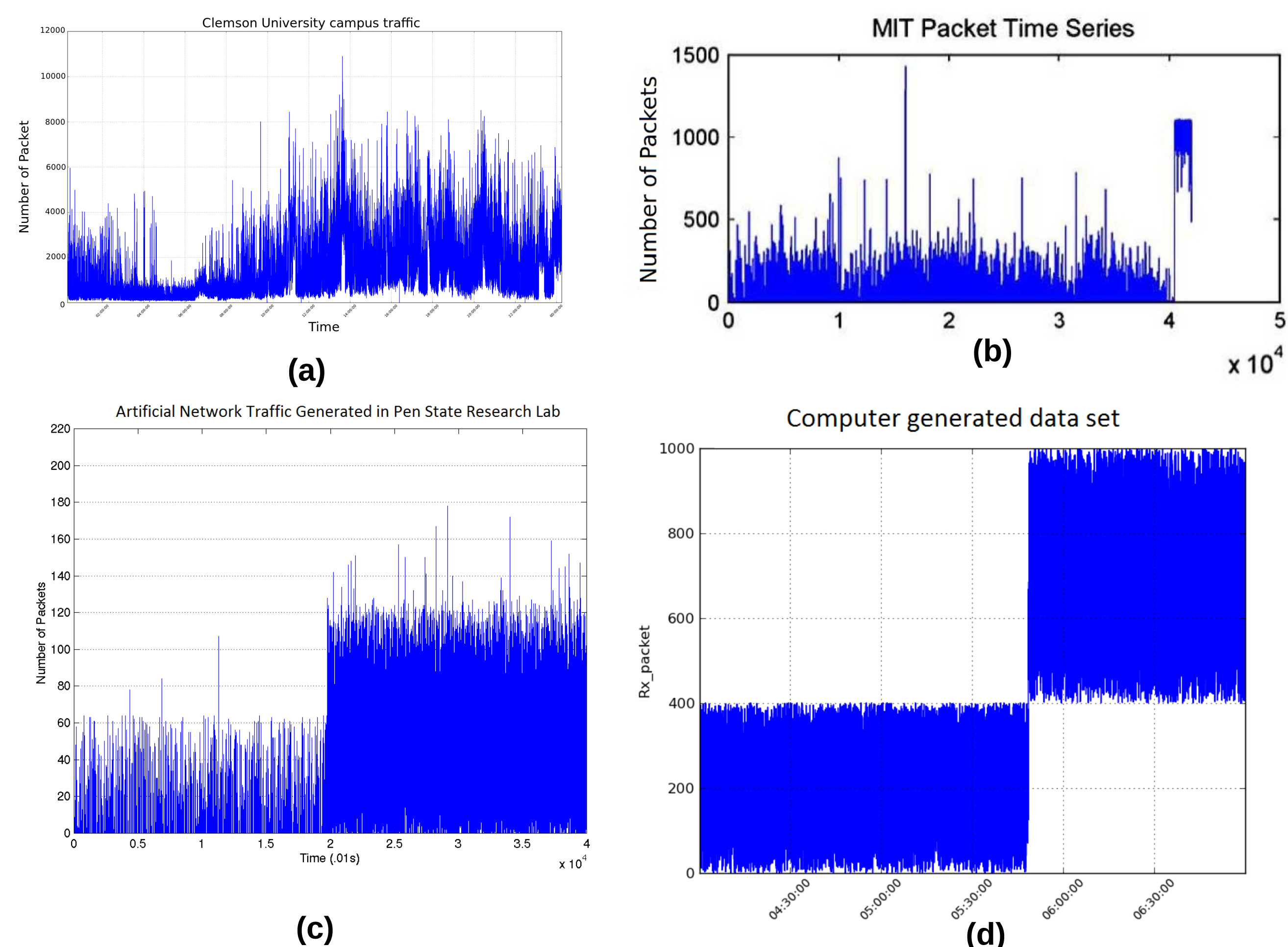
Fig 3. Different kind of network traffic (a) Clemson University campus traffic without attack (b) Artificial network traffic generated MIT lab with attack (c) Artificial network traffic generated in Pen State research lab with attack (d) Dataset generated in Matlab with attack.
