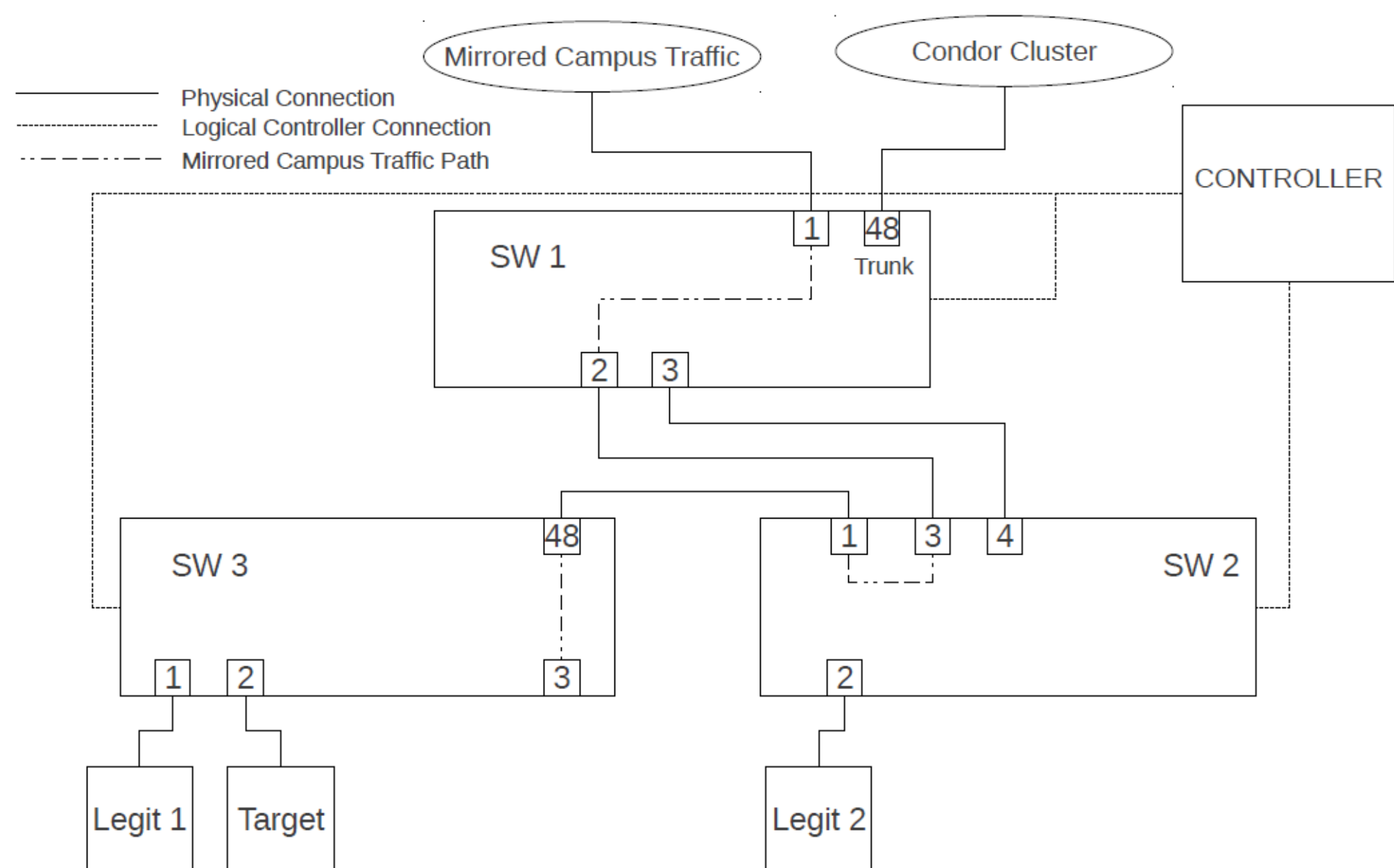
Fig 2. Experiment setup
